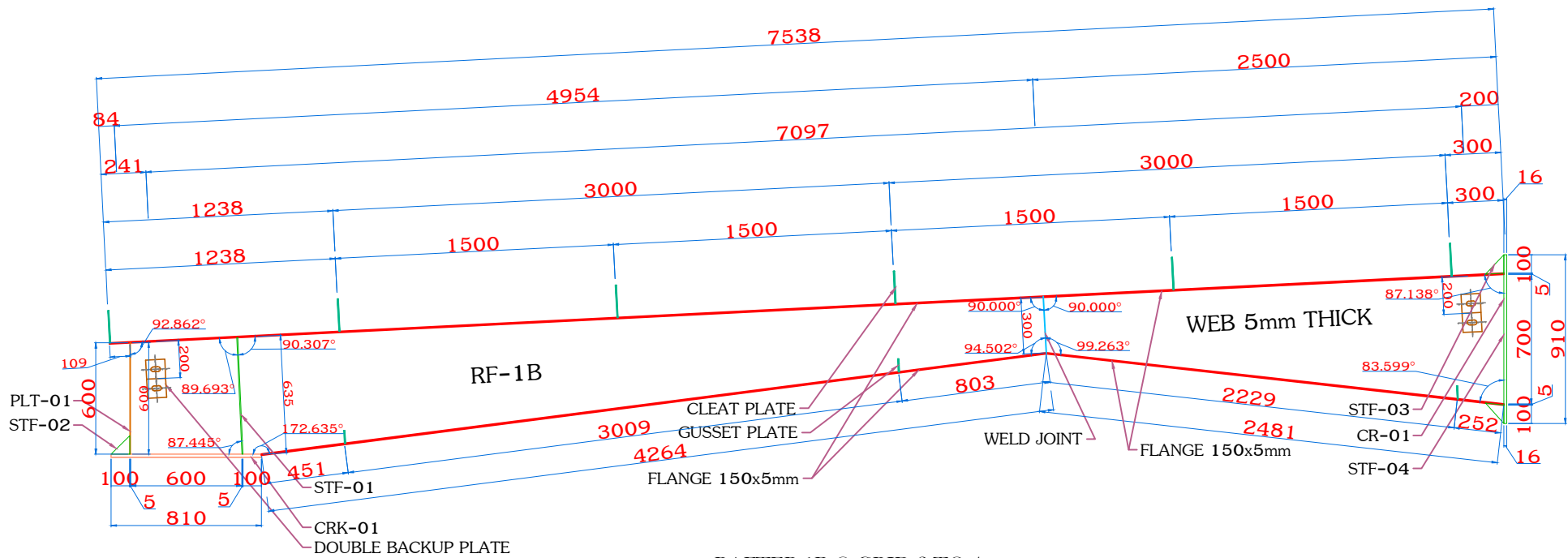
RAFTER-1B @ GRID 2 TO 4 QTY:(03,L)(03,R)
